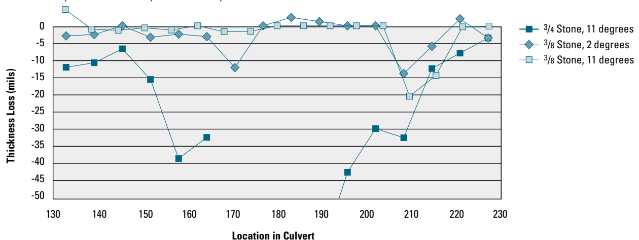
FIGURE 8. Polymer Modified Asphalt Over Polymer Precoat
