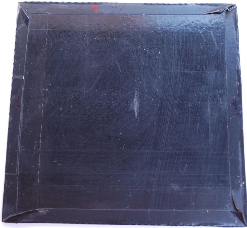
Sample 9B, 100 Cycles, Trenchcoat over galvanized
